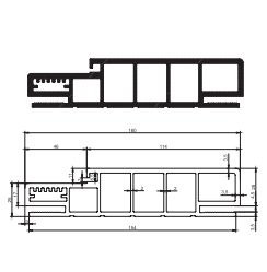
45x90 Pervaz Oval / 45x90 Case Oval
